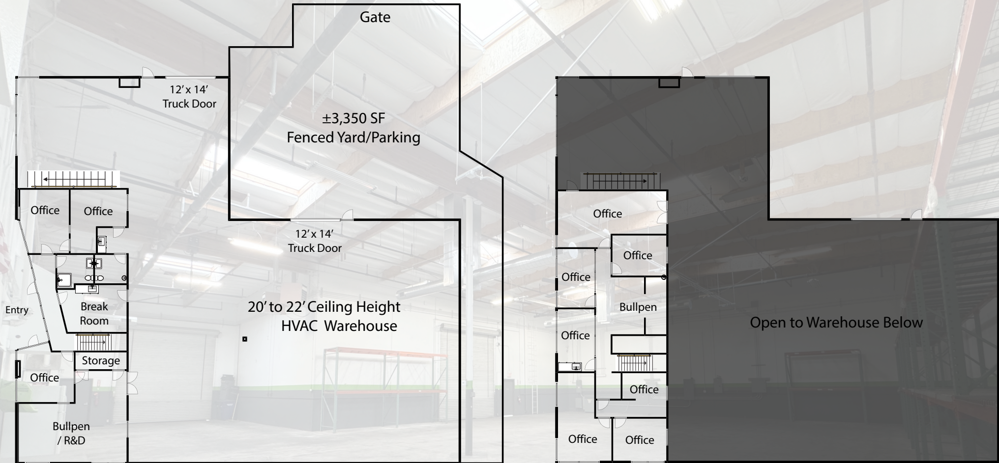
First Floor
